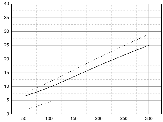
Fig. 8 Switching loss vs. collector current
